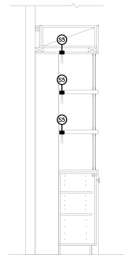
DETAIL G WAITERS STATION SECTION SCALE 1:20
