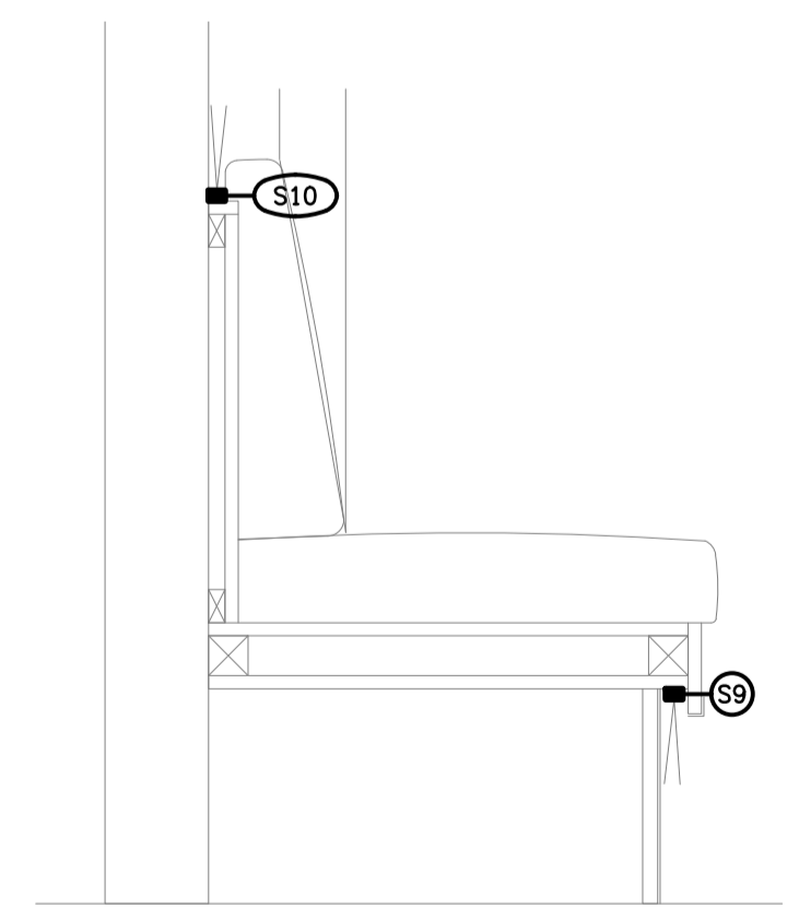
DETAIL H BANQUETTE SEAT SECTION SCALE 1:10
